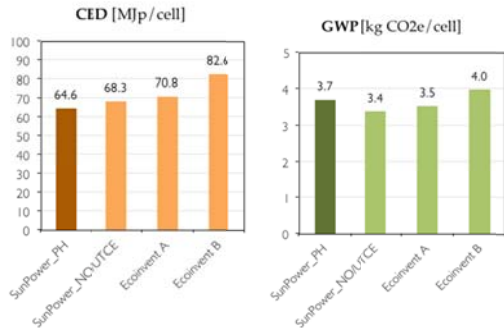
Figure 1: Life cycle impact assessment results in CED and GWP, per cell. (SunPower reference case-Phillipines; SunPower_NO_EU and Ecoinvent B corresponds to MG-Si production in Norway, and balance of production using average (UTCE) European grid electricity)
