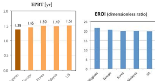
Figure 8: EPBT and EROI of ground-mount systems under average U.S. insolation (1800 kWh/m 2 /yr).
